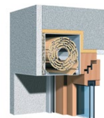
Plaster support variants Behind the stucco – nearly invisible.
